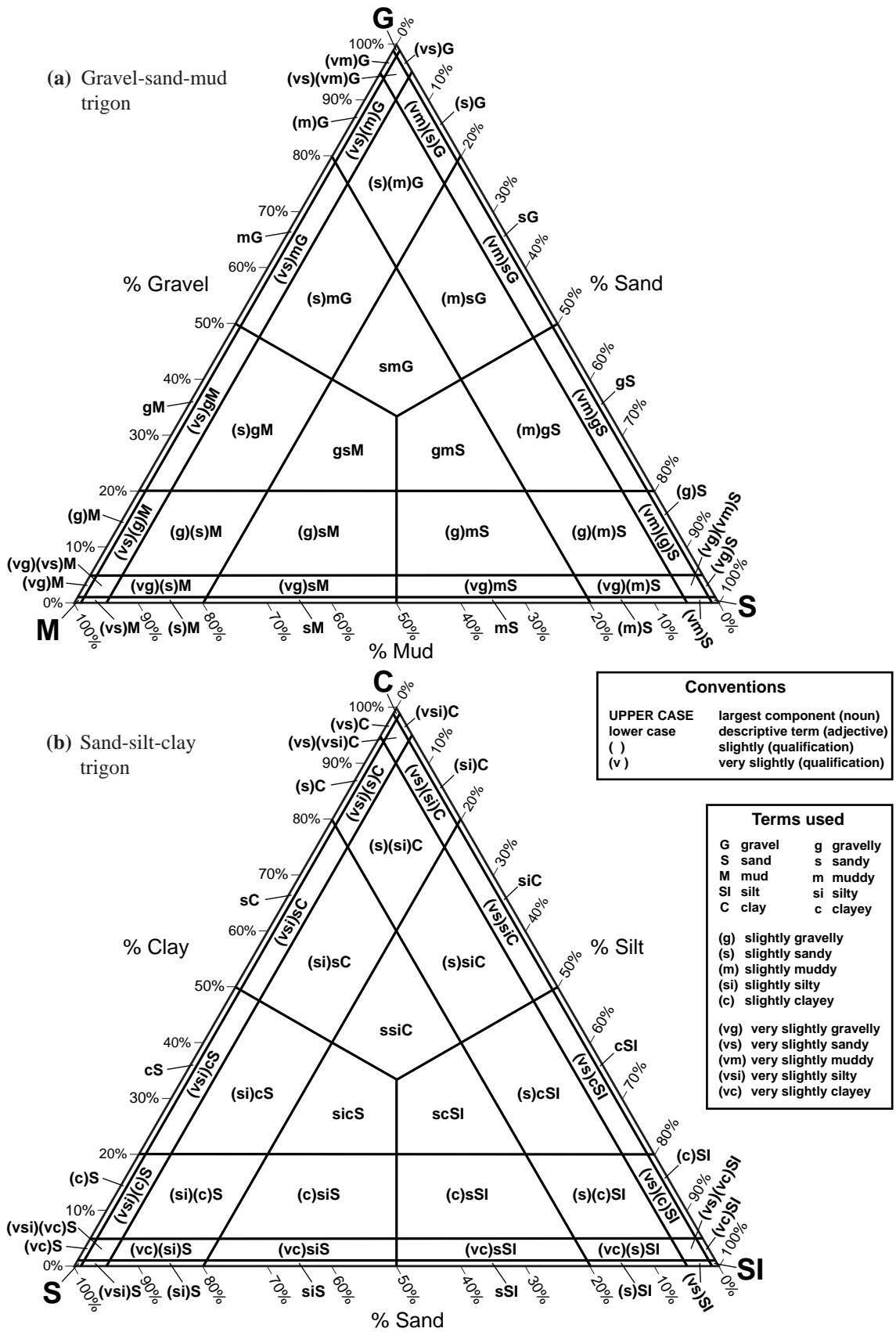
New particle size distribution classifications suggested by Blott and Pye (in press), based on the percentages of (a) gravel, sand and mud (GSM diagram); and (b) sand, silt and clay (SSC diagram).
